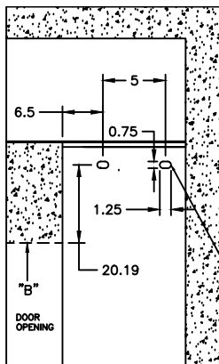
DETAIL A MOUNTING HOLE LOCATIONS
