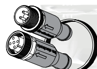
(1) M12 CAN cable PN: 1210855-0X
