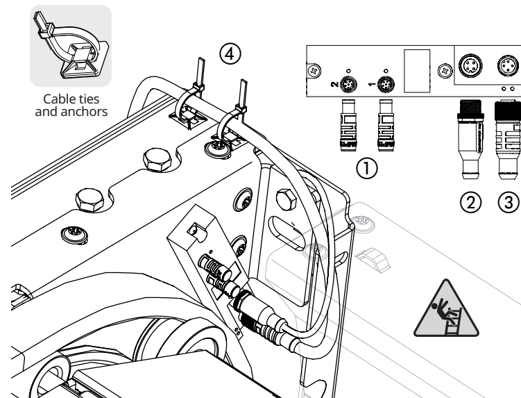
(1) M12 CAN flying lead Cable to controller PN: 1210856-0
