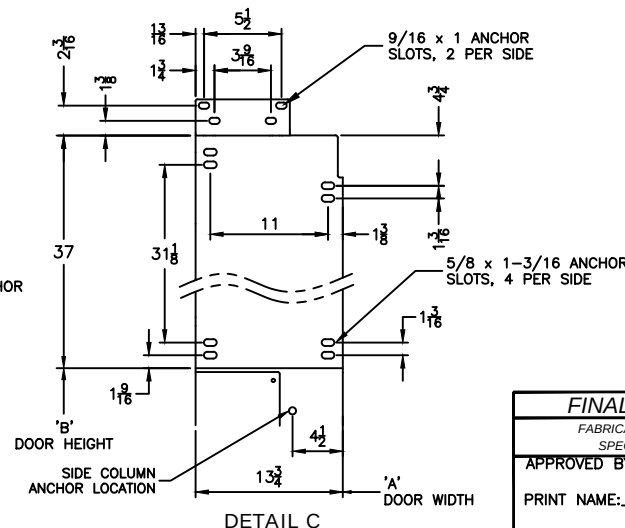
DETAIL C
