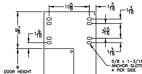
DETAIL C
