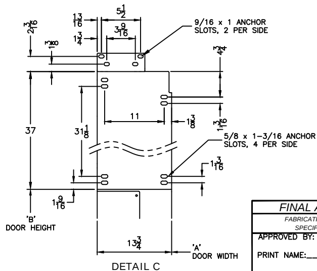
DETAIL C
