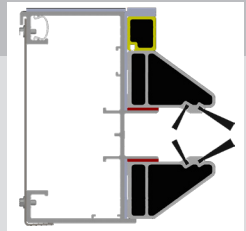
Low profile footprint with integral thermal breaks
