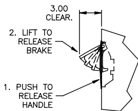
DETAIL A (FRONT VIEW) FLUSH, SIDE MOUNT BRAKE RELEASE HANDLE
