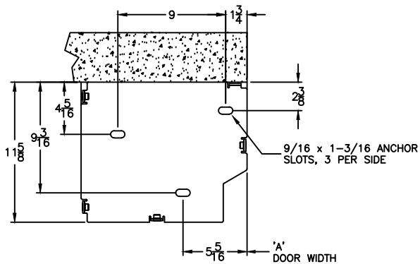
DETAIL B
