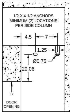
'DETAIL A' MOUNTING HOLE LOCATIONS
